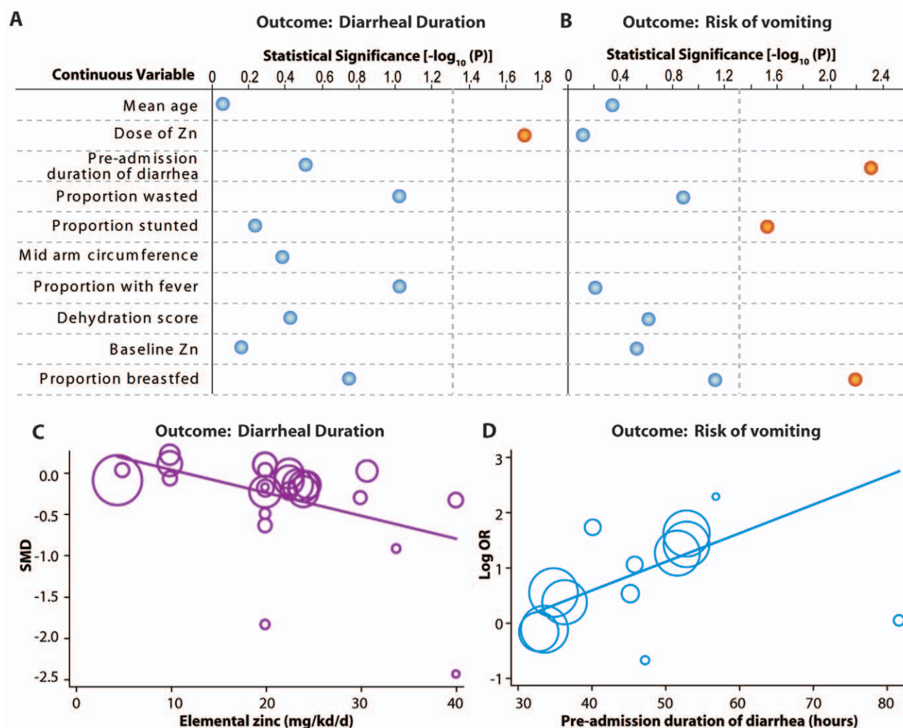
Figure 3. Investigation of the potential contribution of continuous variables to heterogeneity across study results for the outcomes of mean diarrheal duration and risk of vomiting. (A and B) Results from univariate meta-regression for continuous variables as predictors of the between-study heterogeneity for mean diarrheal duration (A) and risk of vomiting (B). The statistical significance is shown as log transformed p-value and the vertical dashed line corresponds to a p-value of 0.05. Blue dots, statistically insignificant; red dot, statistically significant. (C and D) Bubble plots showing the influence of the dose of elemental zinc as a predictor of the standardized mean difference of diarrheal duration (C) and log odds ratio of the risk of vomiting (D). Each bubble represents a study group listed in Figure 2 and the size of the bubble is proportional to the inverse-variance weights.
