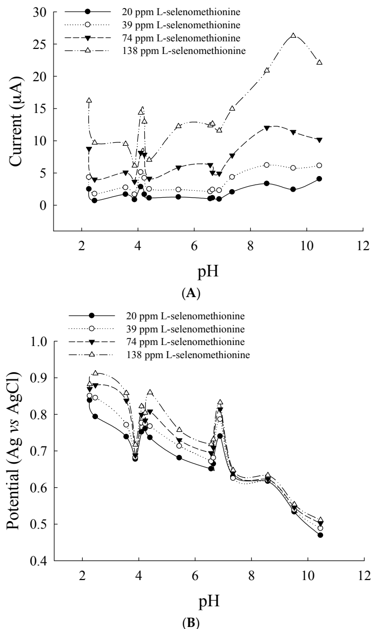
Figure 2. Effect of pH values on anodic peak in Britton and Robison buffer (pH 2.46–10.45) containing 20–138 \text{mg}\cdot\text{L}^{-1} L-selenomethionine. (A) The relationships between peak currents and pH and (B) the relationships between potential and pH.
