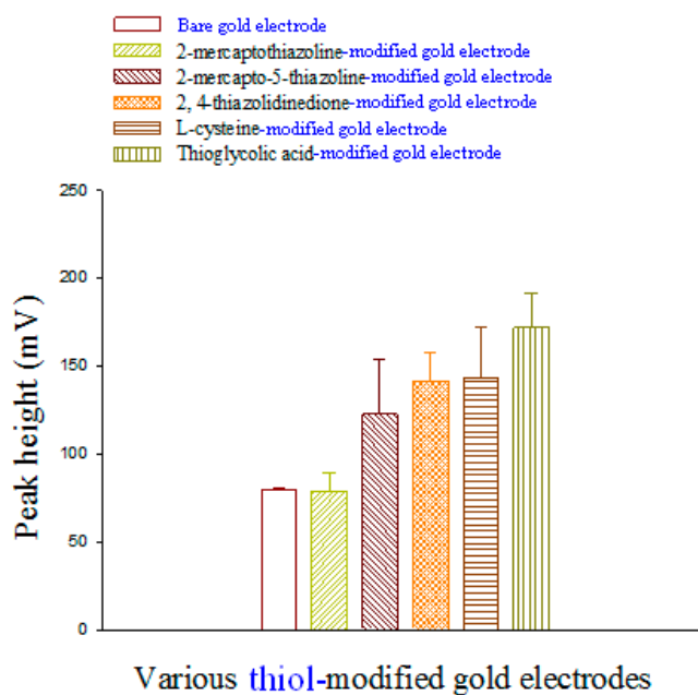
Figure 4. A comparison of a bare Se-methylselenocysteine ( 0.4 \text{ mg} \cdot \text{L}^{-1} ) gold electrode and various Se-methylselenocysteine ( 0.4 \text{ mg} \cdot \text{L}^{-1} ) thiol/Au electrodes in a flow-through voltammetric sensor; the mobile phase is methanol-water (10:90, v/v).
