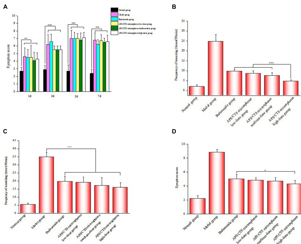
FIGURE 4 | Evaluation of symptom after nasal administration. (A) Results of symptom score evaluation in molding stage (mean \pm SD, n = 10 , **p < 0.01 , ***p < 0.001 ). (B) Frequency of sneezing of rats after nasal administration (mean \pm SD, n = 10 , ***p < 0.001 ). (C) Frequency of scratching of rats after nasal administration (mean \pm SD, n = 10 , ***p < 0.001 ). (D) Results of symptom score evaluation after nasal administration (mean \pm SD, n = 10 , *p < 0.05 ).
