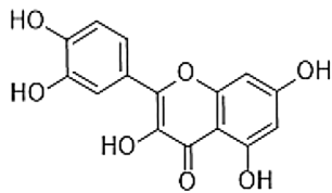
Fig. 1 Structure of quercetin
