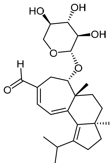
Figure 1. Chemical structure of erinacine A.
