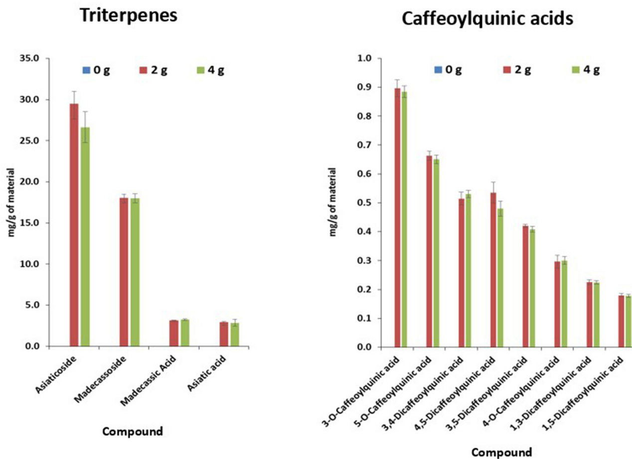
FIGURE 3 | Concentration of triterpenes and caffeoylquinic acids found in 0, 2, and 4 g Centella asiatica product as determined by LC-HRMS. Sachets of the Centella asiatica water extract products (CAP; n = 5 per dose) were extracted with methanol and analyzed for the content of active compounds (triterpenes and caffeoylquinic acids) using LC-HRMS in positive and negative ion mode against commercial reference standards. The content of triterpenes and caffeoylquinic acids per gram of Centella asiatica extract was identical for the 2 g and 4 g doses of CAP and showed low variability indicating successful and uniform manufacture of the two doses. None of the specific analytes were detected in the 0 g dose, confirming their absence at detectable levels in the placebo which was comprised solely of the excipients used.
