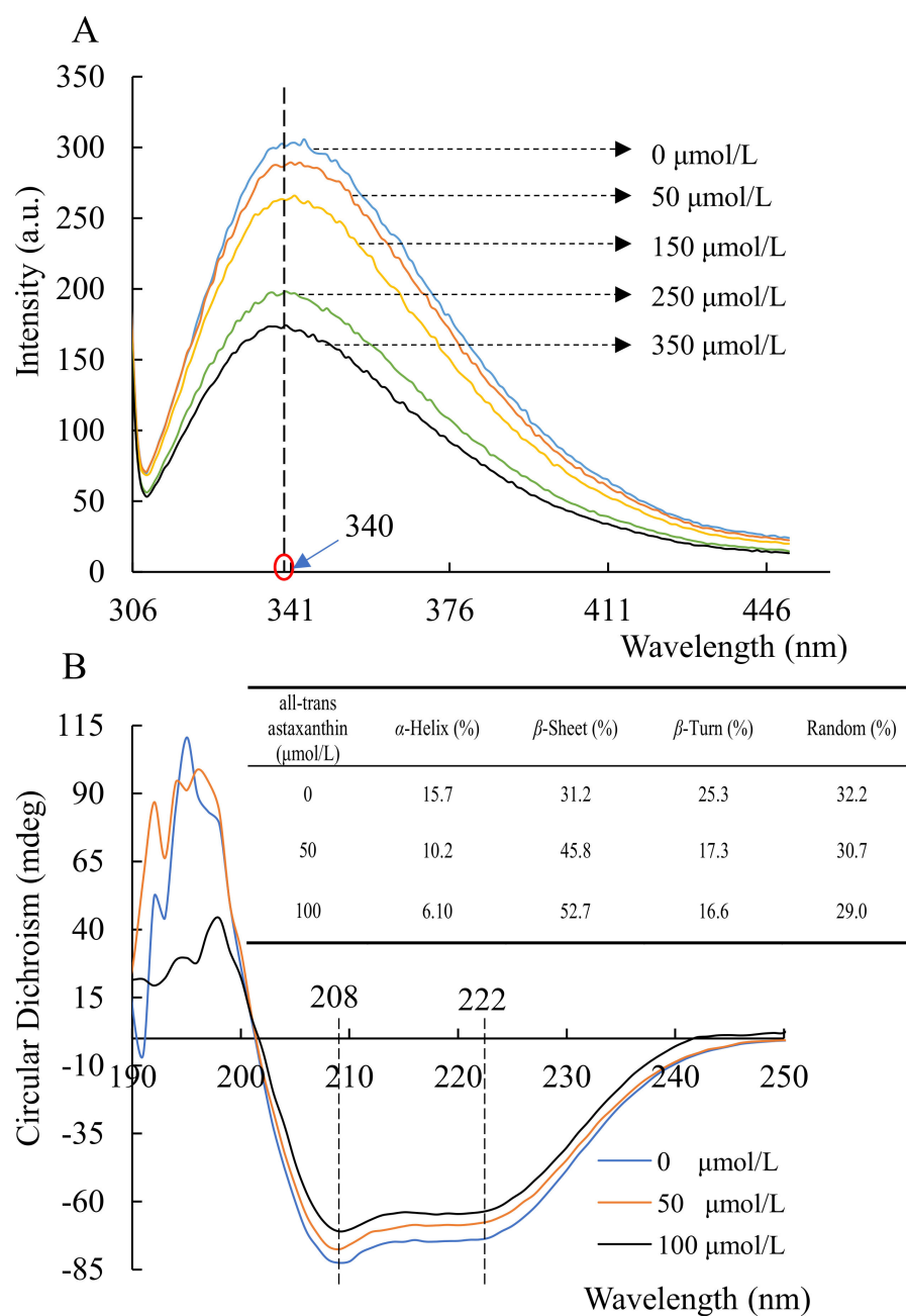
Figure 3. Fluorescence emission (A) and circular dichroism (B) spectra of acetylcholinesterase in the presence of all-trans astaxanthin with various concentrations.
