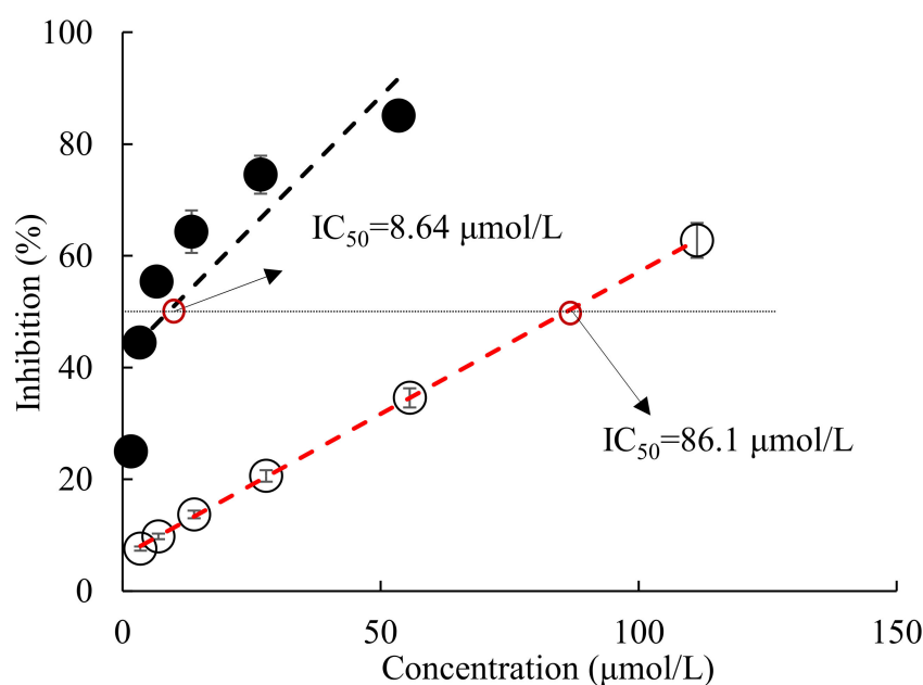
Figure 1. Inhibition of acetylcholinesterase by all-trans astaxanthin and galantamine. ●: all-trans astaxanthin; ○: galantamine.
