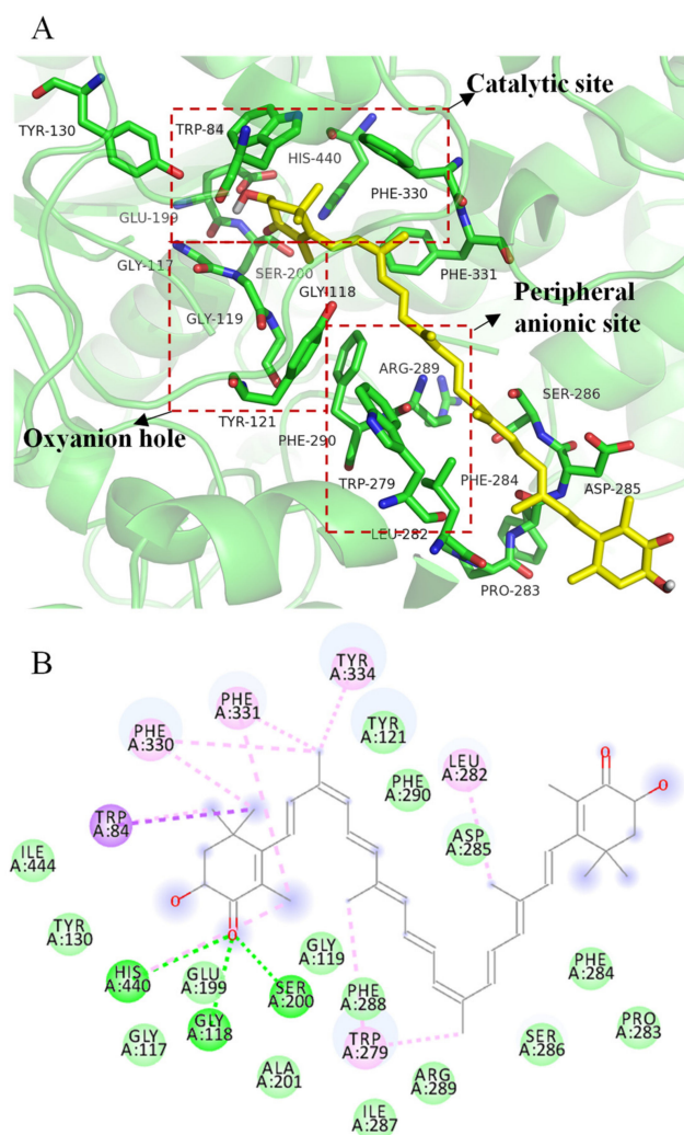
Figure 6. 3D (A) and 2D (B) structural simulation of all-trans astaxanthin interacting with acetylcholinesterase.
