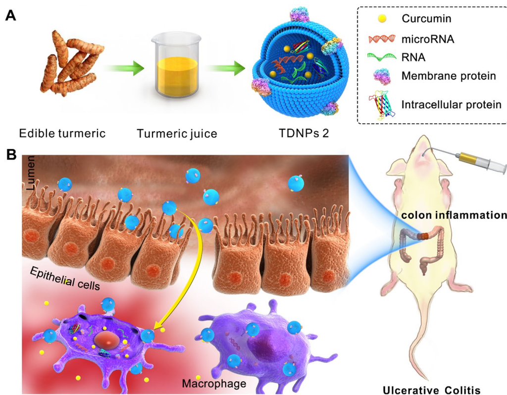
Fig. 1 Schematic illustration of turmeric-derived nanoparticles (TDNPs 2) isolation and targeted ulcerative colitis (UC) therapy via oral administration. A TDNPs 2 were isolated and purified from edible turmeric by ultracentrifugation and sucrose gradient centrifugation. B By oral administration, TDNPs 2 accumulated at inflamed colon and exerted UC therapeutic effect
