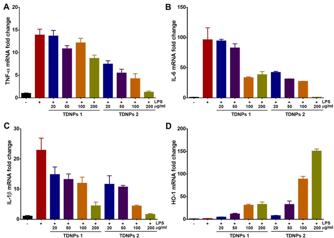
Fig. 3 TDNPs prevent LPS-induced macrophage inflammation. A–C mRNAs expression of pro-inflammatory cytokines, TNF- \alpha , IL-6 and IL-1 \beta , respectively (n = 5). D mRNA expression of HO-1 (n = 5)
