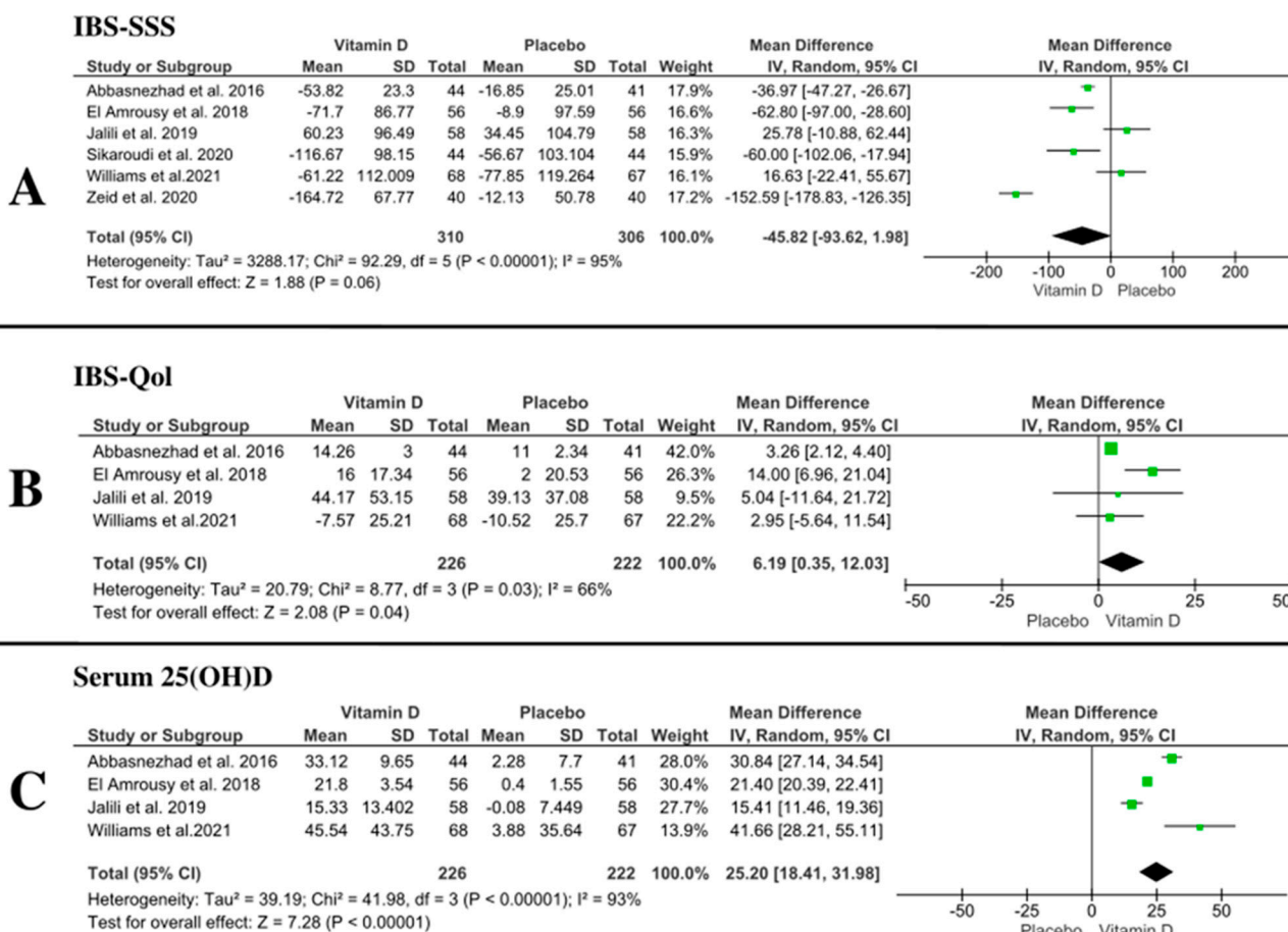
Figure 3. Forest plot of the included outcomes ((A)—IBS-SSS, (B)—IBS-QoL, (C)—serum 25(OH)D). I 2 : I-squared; CI: confidence interval [27–32,43].
