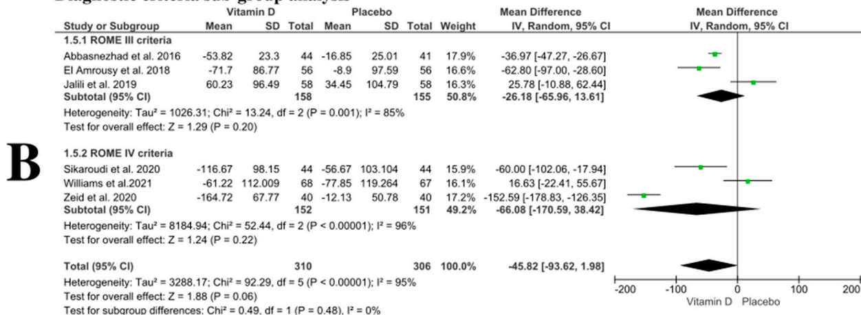
Figure 4. Forest plot of the sub-group analysis ((A)—dosage sub-group analysis, (B)—diagnostic criteria sub-group analysis) I 2 : I-squared; CI: confidence interval [27–32,43].
