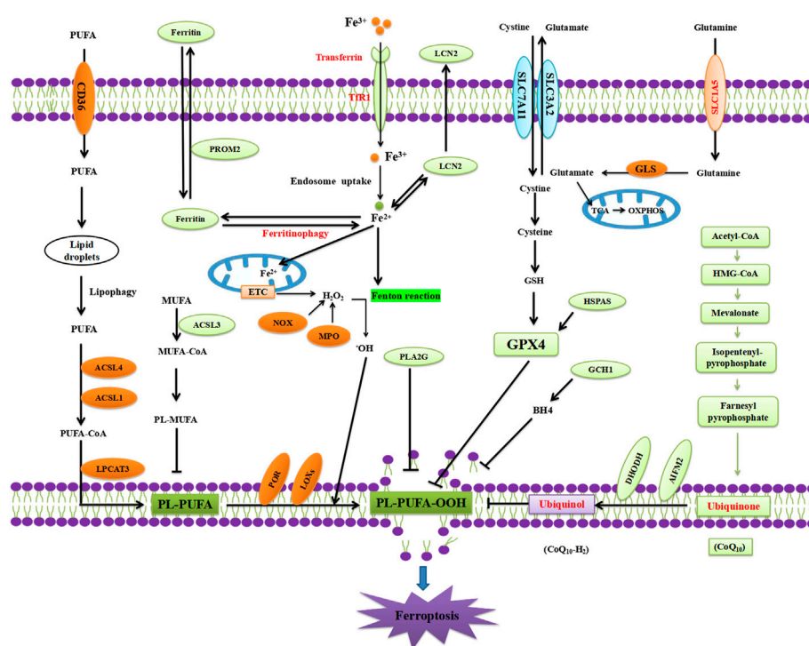
FIGURE 3 Mechanism of ferroptosis.
