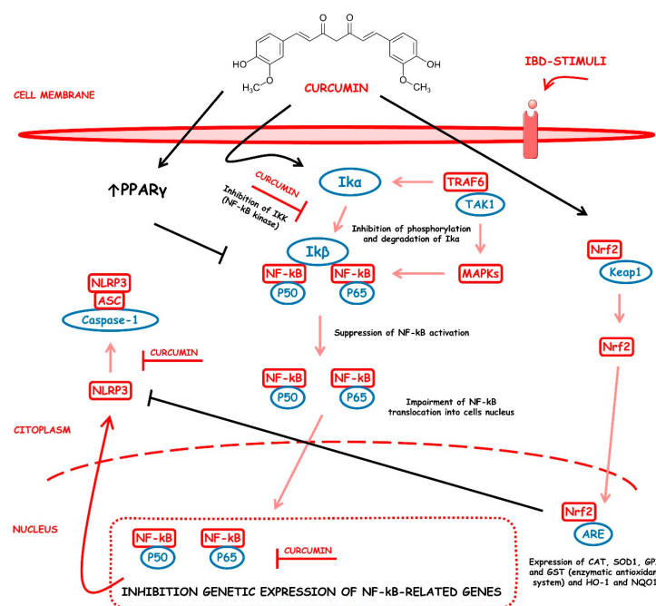
Figure 2. NF-κB regulation with the use of curcumin. ↑, increase; ARE, antioxidant response elements; ASC, apoptosis-associated Speck-like protein; CAT, catalase; HO-1, heme oxygenase 1; GPX, glutathione; GST, glutathione S-transferases; IBD, inflammatory bowel diseases; Keap1, Kelch-like ECH-associated protein 1; MAPK, mitogen-activated protein kinases; NF-κB, nuclear factor-Kb; NLRP3, NLR (/nucleotide-binding leucine-rich repeat receptor) family pyrin domain containing 3; NQO1, NAD(P)H dehydrogenase (quinone) 1; Nrf2, nuclear factor erythroid 2–related factor 2; SOD1, superoxide dismutase 1; TAK1, transforming growth factor-β-activated kinase 1; TRAF6, tumor necrosis factor receptor (TNFR)-associated factor 6.
