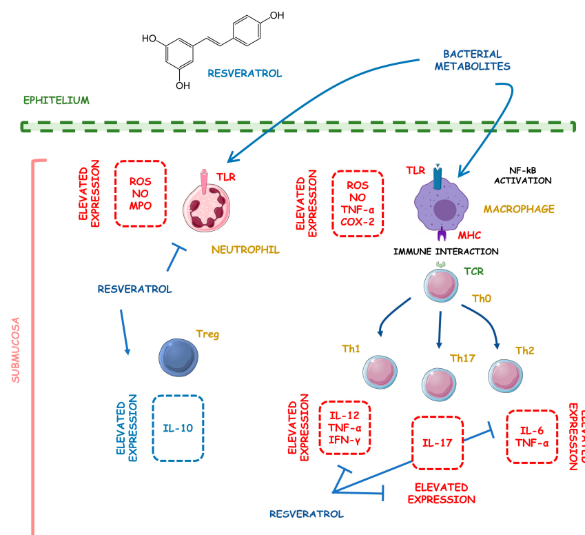
Figure 3. Main regulatory effects of RSV on NF-κB modulation during IBD. IL-6, interleukin 6; IL-10, interleukin 10; IL-12, interleukin 12; IL-17, interleukin 17; MHC, major histocompatibility complex; MPO, myeloperoxidase; NF-κB, nuclear factor-κB; NO, nitric oxide; ROS, reactive oxygen species; TCR, T-cell receptor; Th0, T helper 0; Th1, T helper 1; Th2, T helper 2; Th17, T helper 17; TLR, Toll-like receptor; TNF-α, tumor factor necrosis alpha; Treg, regulatory T cell.
