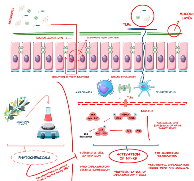
Figure 1. Inflammatory bowel diseases (IBD), activation of the nuclear factor- \kappa B (NF- \kappa B), and the possible roles of phytochemicals against this pathway activation during these diseases. \uparrow , increase; TLRs, Toll-like receptors; IKK \alpha , IkappaB kinase alpha; IKK \beta , IkappaB kinase beta; IKB, inhibitor of nuclear factor- \kappa B.
