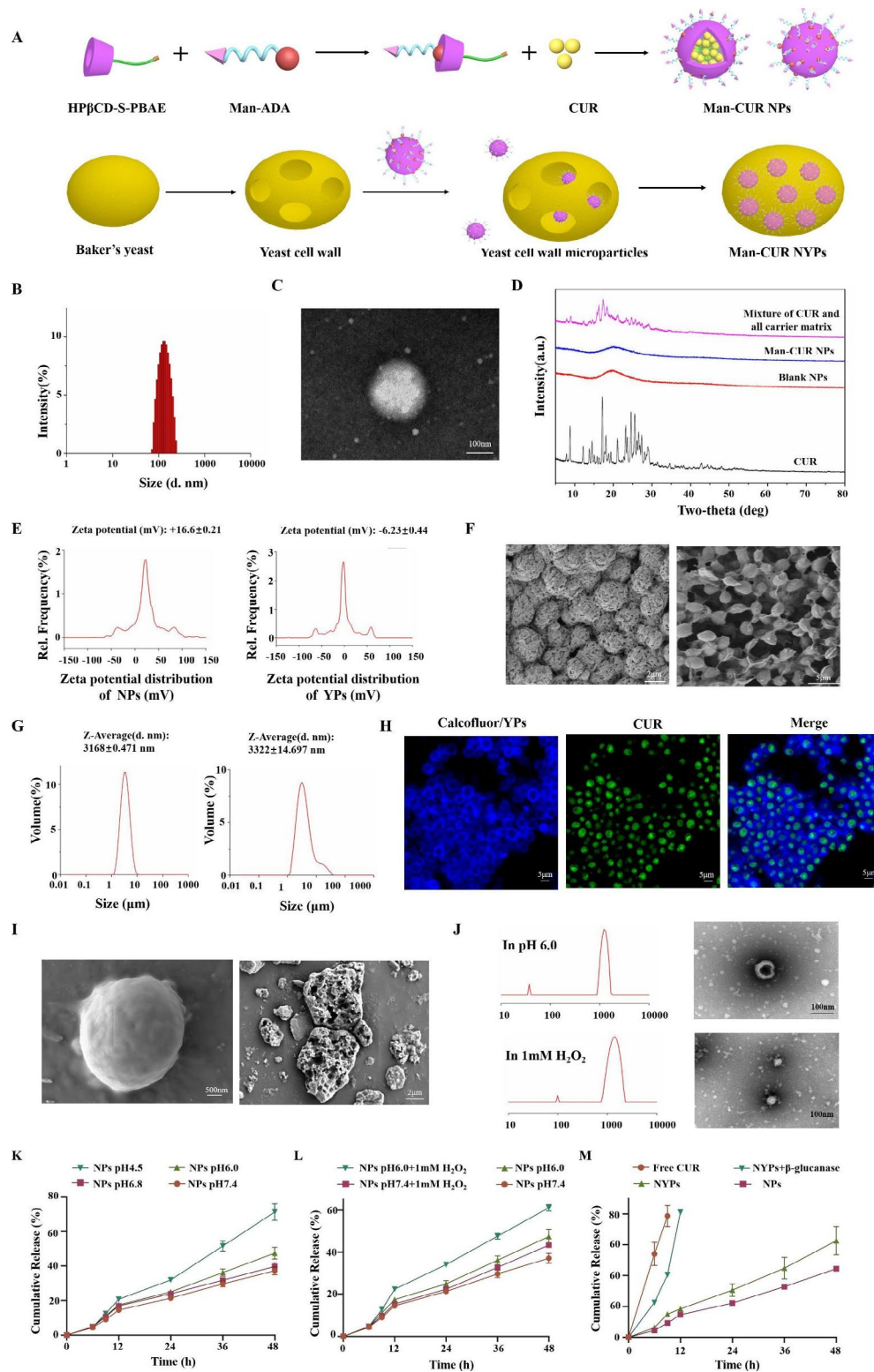
Fig. 2 Characterization, stability, and release behavior of Man-CUR NPs and Man-CUR NYPs: (A) Fabrication process of Man-CUR NPs and Man-CUR NYPs. (B) Size distribution of Man-CUR NPs. (C) TEM image of Man-CUR NPs. (D) XRD analysis. (E) Zeta potential distribution of NPs and YPs. (F) SEM image of YPs and Man-CUR NYPs. (G) Size distribution of YPs and Man-CUR NYPs. (H) Representative CLSM images of Man-CUR NPs (green) and the yeast cell wall was labeled with calcofluor white (blue; scale bar = 25 \mu m). (I) Stability evaluation of NYPs. (J–M) The size distribution, TEM and cumulative release profiles of CUR under different conditions. Data are shown as means \pm SD ( n=3 )
