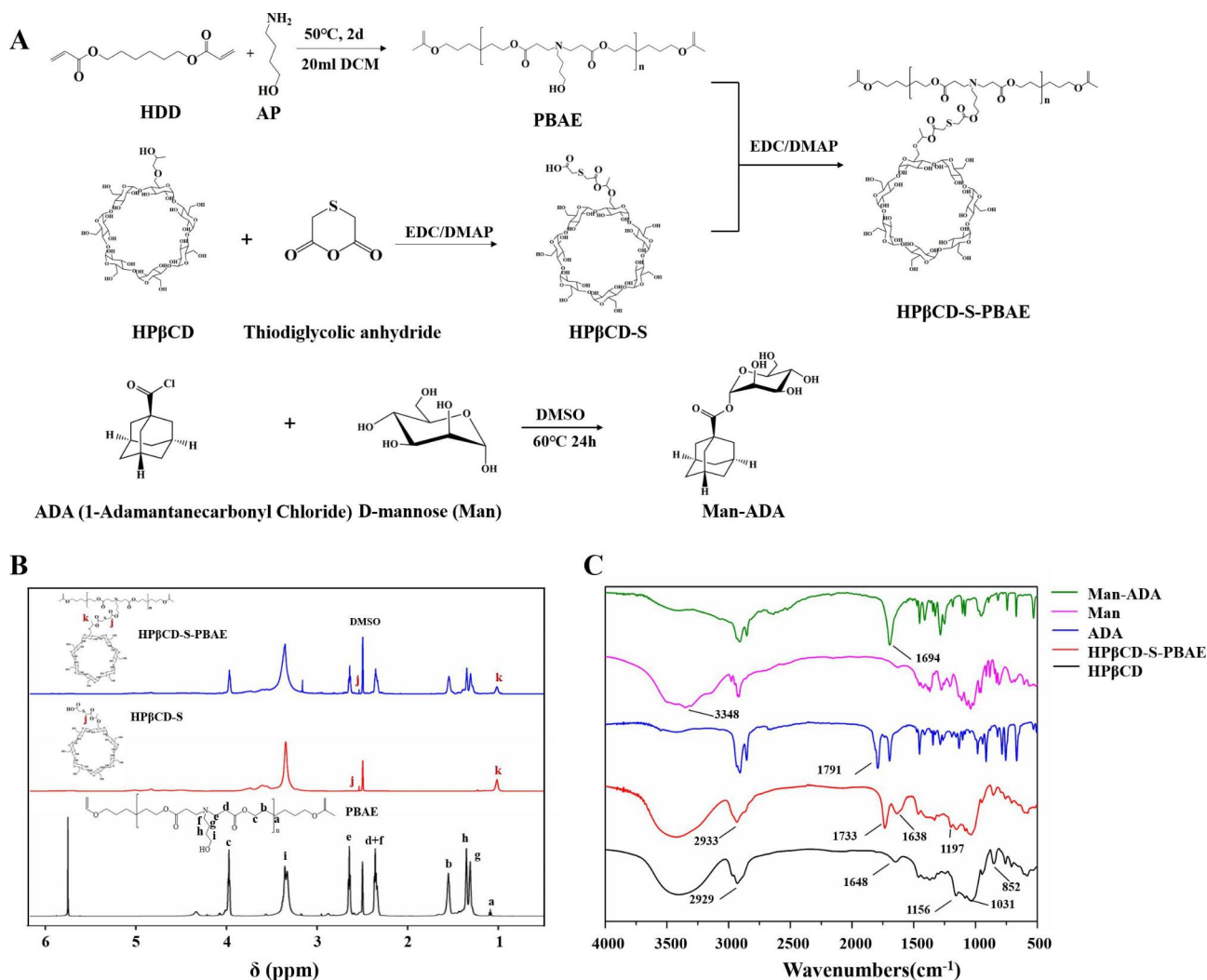
Fig. 1 Copolymer synthesis and characterization: (A) Synthesis route of HP \beta CD-S-PBAE and Man-ADA. (B) ^1\text{H} NMR spectra of HP \beta CD-S-PBAE. (C) FTIR spectra of HP \beta CD-S-PBAE and Man-ADA.
