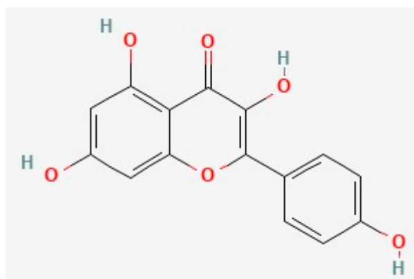
Figure 3. The chemical structure of kaempferol, deduced from PubChem [202].
