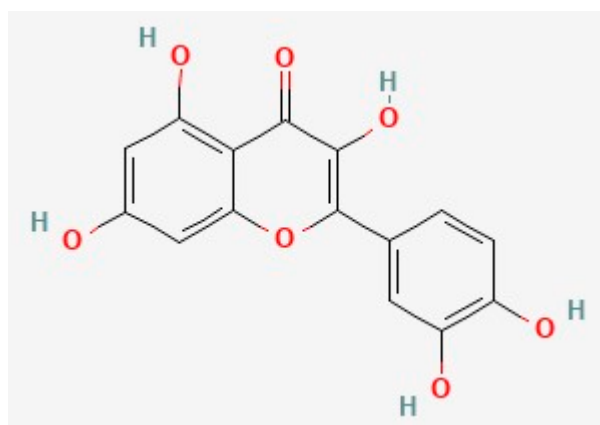
Figure 2. The chemical structure of quercetin, deduced from PubChem [164].
